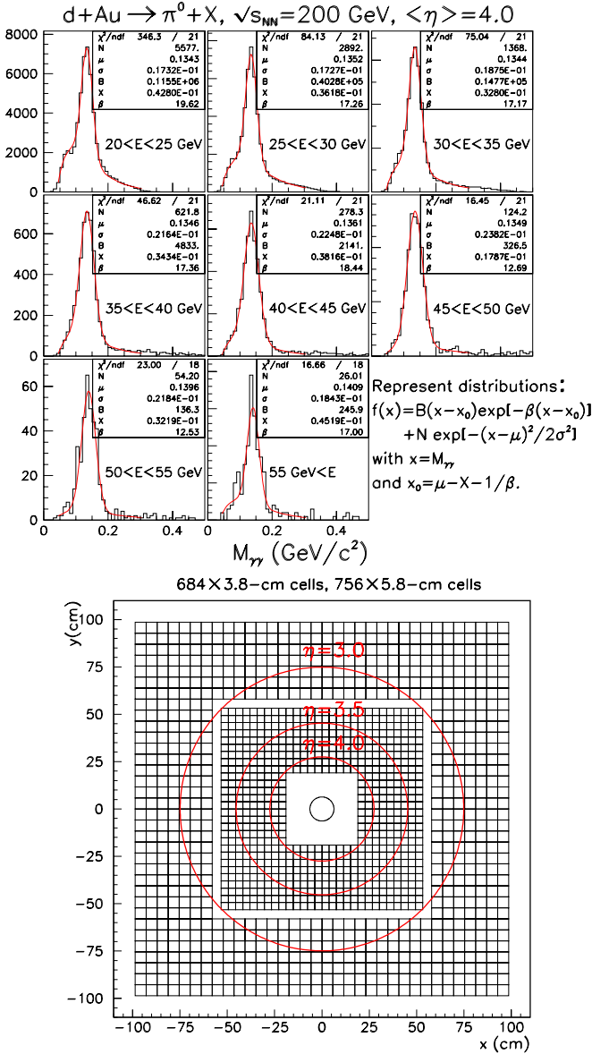
Fig. 6. Top: Di-photon invariant mass distributions from the STAR FPD for d+Au collisions at \sqrt{s_{NN}}=200 \text{ GeV} at \langle \eta \rangle = 4.0 relative to the incident deuteron beam. Bottom: Layout of the proposed FMS
